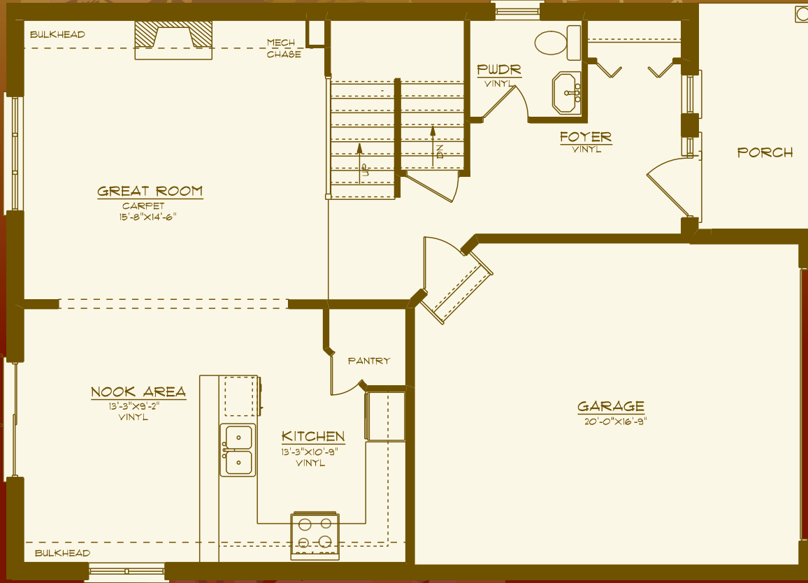
Main Floor 827 Sq. Ft.
